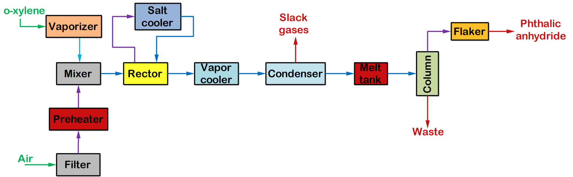
Figure: Manufacture of Phthalic anhydride from o-xylene
